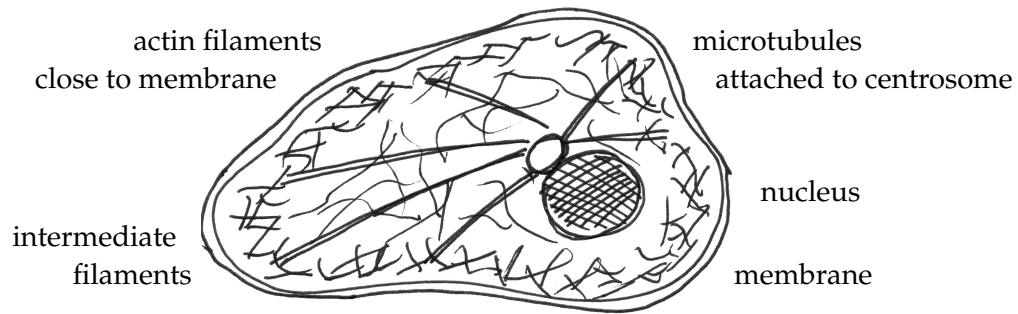
Figure 1.3: Eukaryotic cytoskeleton, consisting of thin actin filaments and intermediate filaments which act as tensile ropes and thick hollow microtubules which act as compressive trusses
