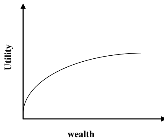
Figure 6.1 Utility Function
