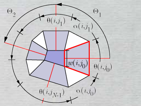
Non intersection (convexity of molecule)
