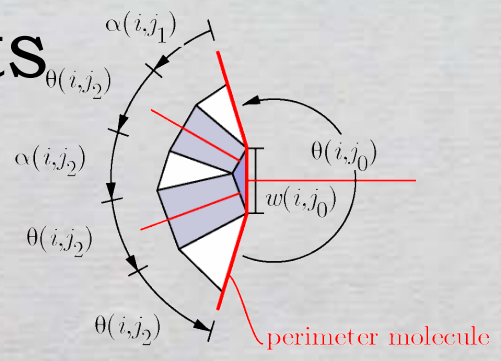
convexity of paper
