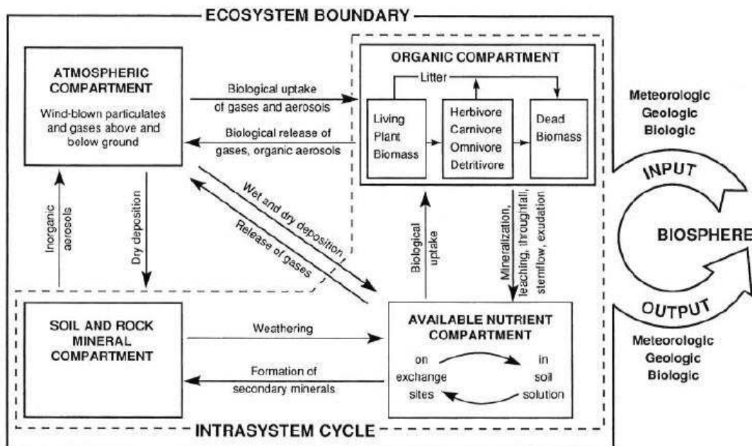
Figure 1.3. Model depicting nutrient relationships in a terrestrial ecosystem. Inputs and outputs to the ecosystem are moved by meteorologic, geologic and biologic vectors (Bormann and Likens 1967, Likens and Bormann 1972). Major sites of accumulation and major exchange pathways within the ecosystem are shown. Nutrients that, because they have no prominent gaseous phase, continually cycle within the boundaries of the ecosystem between the available nutrient, organic matter and primary and secondary mineral components tend to form an intrasystem cycle. Fluxes across the boundaries of
