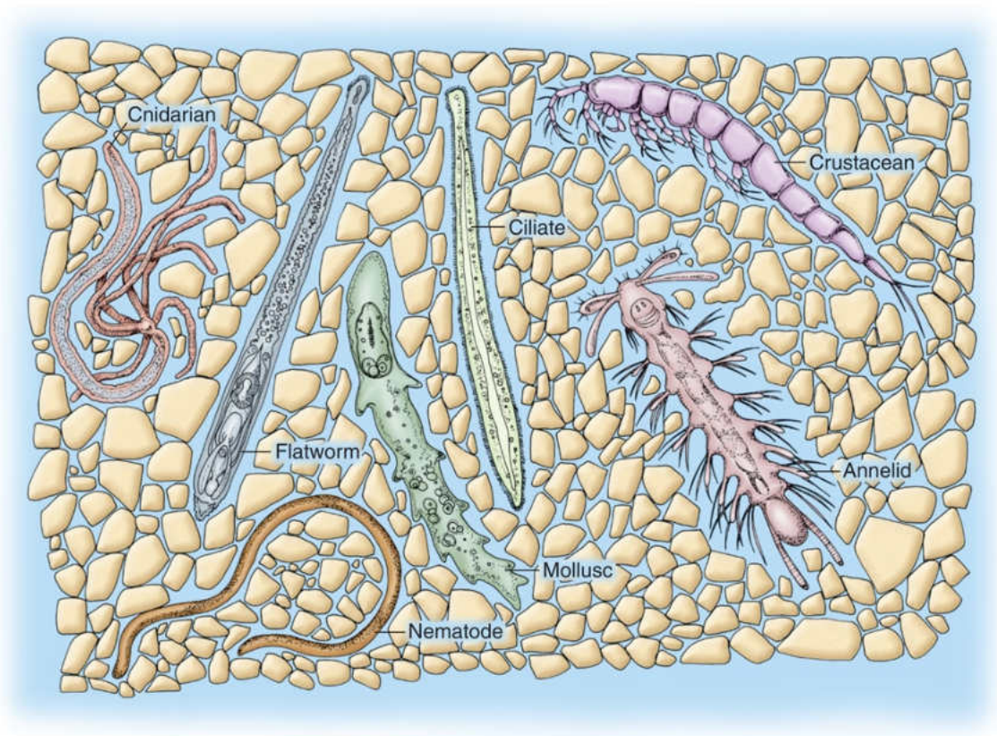
Figure 12.5. Typical meiofauna.
