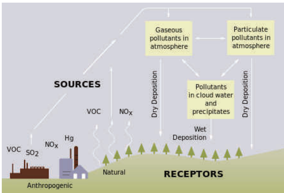
Figure 1. Processes involved in acid deposition.
