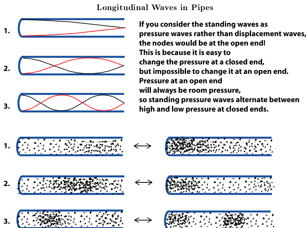
Figure 3.11: The standing waves in the tubes are actually longitudinal sound waves. Here the displacement standing waves in Figure 3.10 (Standing Waves in Wind Instruments) are shown instead as longitudinal air pressure waves. Each wave would be oscillating back and forth between the state on the right and the one on the left. See Standing Waves in Wind Instruments 17 for more explanation.
