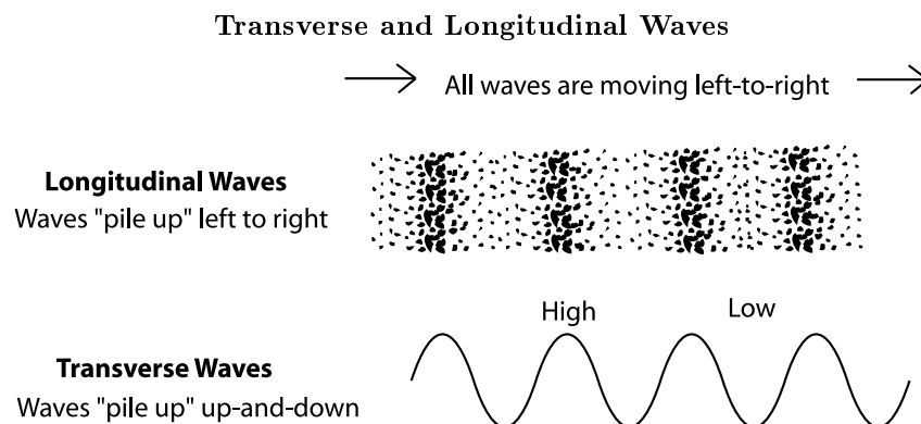
Figure 3.2: In water waves and other transverse waves , the ups and downs are in a different direction from the forward movement of the wave. The "high and lows" of sound waves and other longitudinal waves are arranged in the "forward" direction.
